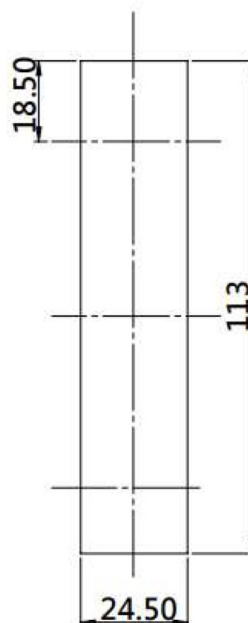
CUT OUT
